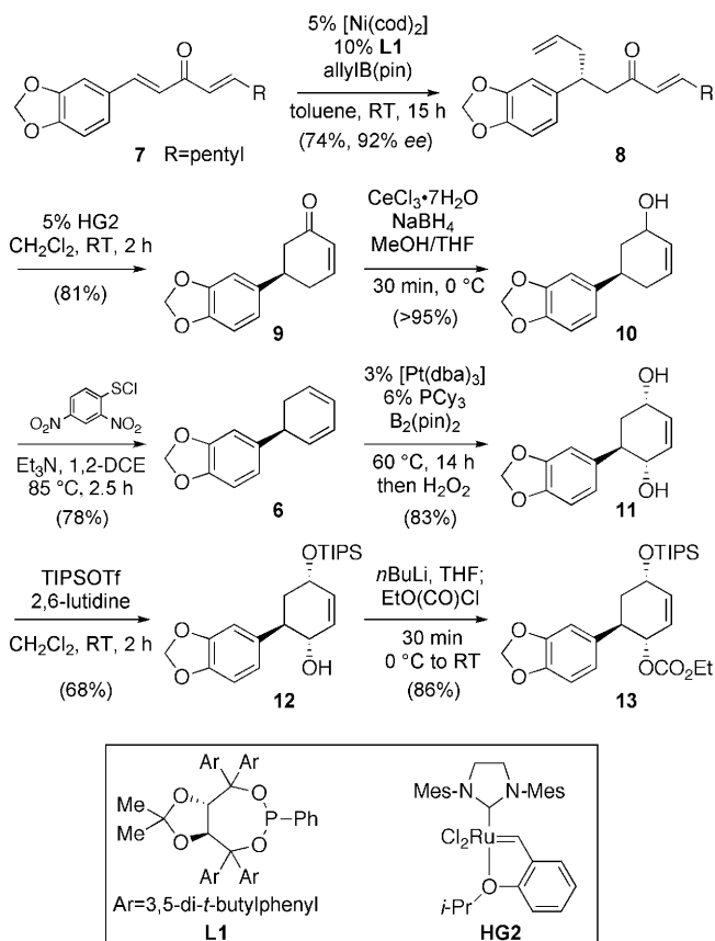
Scheme 2. Synthesis of 13 . cod = 1,5-cyclooctadiene, DCE = dichloroethane, Mes = 2,4,6-trimethylphenyl, Tf = trifluoromethanesulfonyl, THF = tetrahydrofuran, TIPS = triisopropylsilyl.
